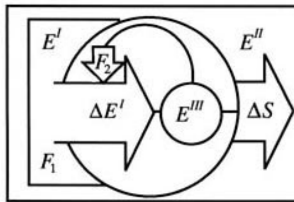
Figure 3. A generalized autocatakinetic system. E^I and E^{II} indicate a source and a sink with the difference between them constituting a field potential with a thermodynamic force F_1 (a gradient of a potential) the magnitude of which is a measure of the difference between them. \Delta E^I is the energy flow at the input, the drain on the potential which is transformed into entropy production \Delta S at the output. E^{III} is the internal potential carried in the circular relations that define the system by virtue of its distance from equilibrium that acts back to amplify or maintain input during growth or non-growth phases respectively with an internal force F_2 . From "Emergent Attractors and the Law of Maximum Entropy Production: Foundations to a General Theory of Evolution" by R. Swenson, 1989b, Systems Research , 6, p. 191. Copyright 1989 by Pergamon. Adapted by permission.
