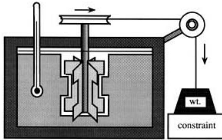
Figure 6. Experiment devised by Joule to show the conservation of energy. When a constraint is removed potential energy in the form of a suspended weight is converted into the mechanical or kinetic energy of a moving paddle wheel in an energy-tight container of water heating the water by an amount consistent with the amount of potential energy lost by the falling weight.
